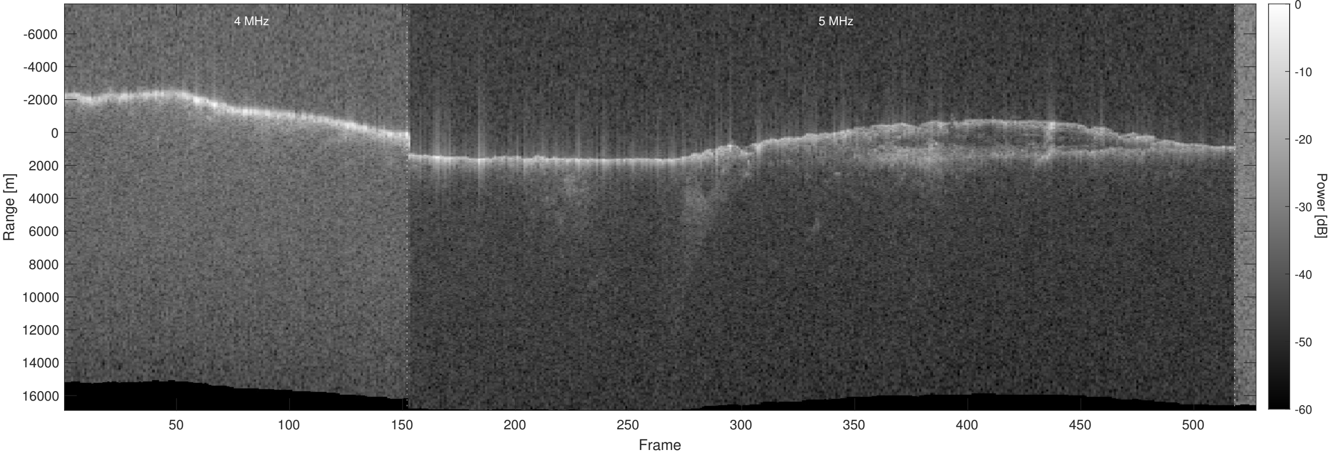
Orbit 5583, Optimized, No Window, Depth-Corrected, Channel 2
