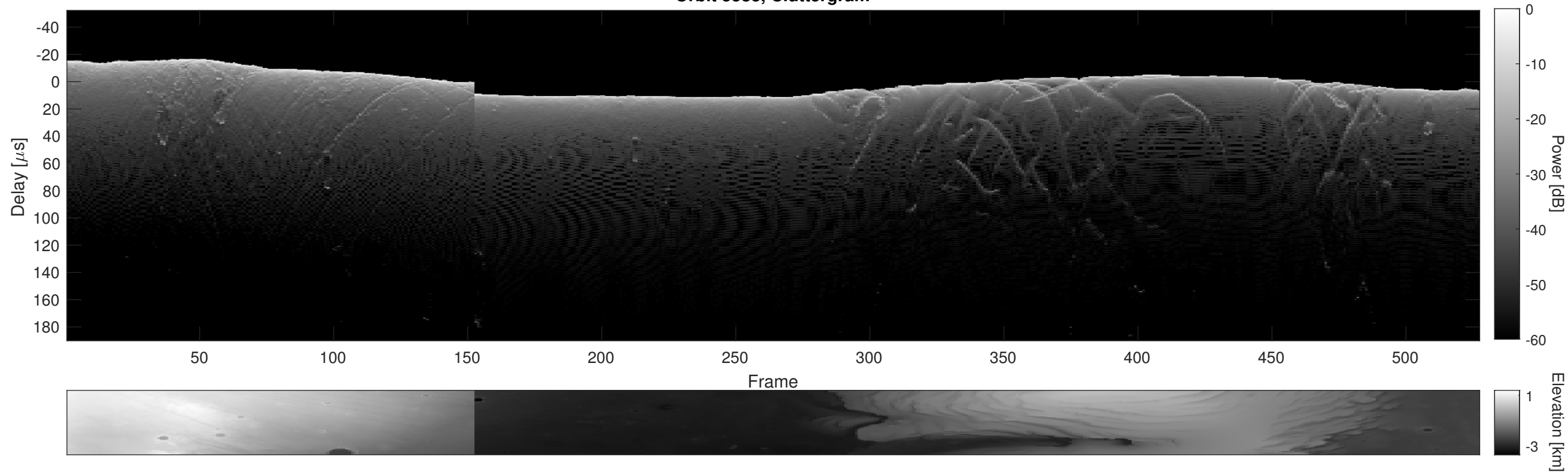
Orbit 5583, Cluttergram
