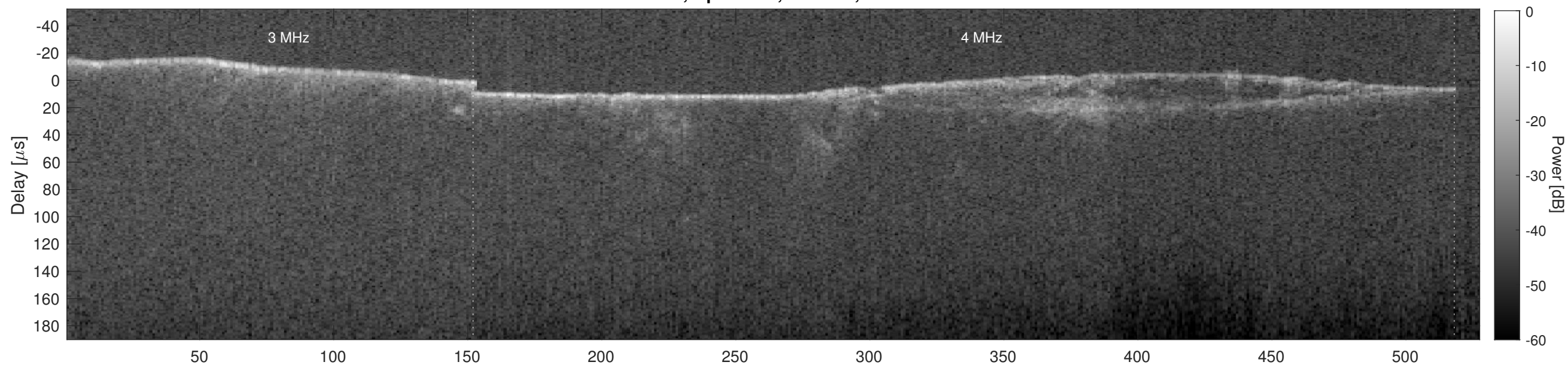
Orbit 5583, Cluttergram
