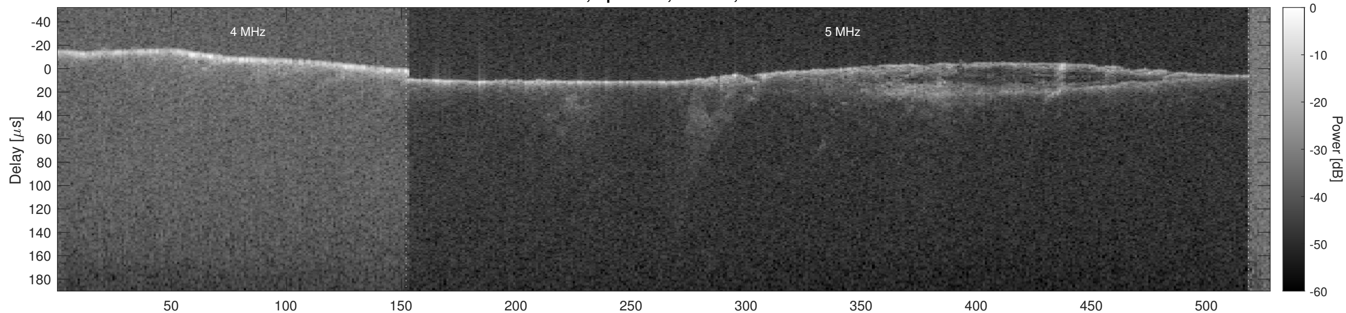
Orbit 5583, Optimized, Window, Channel 2
