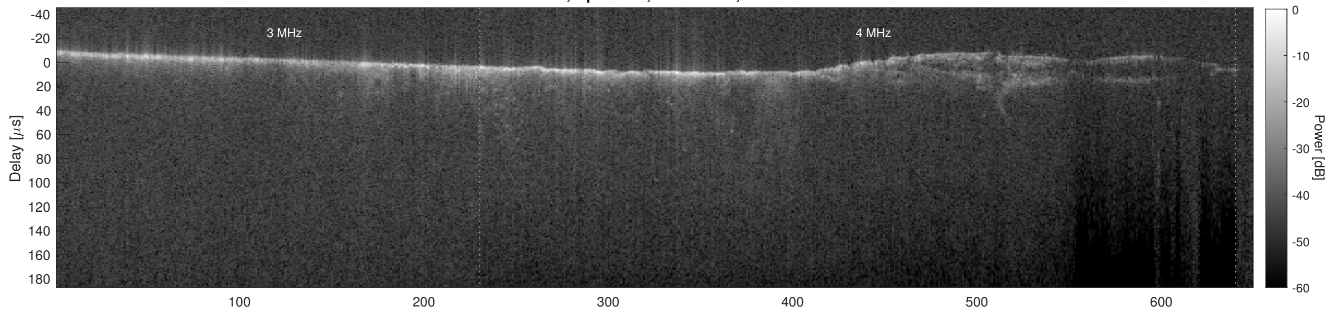
Orbit 5587, Cluttergram
