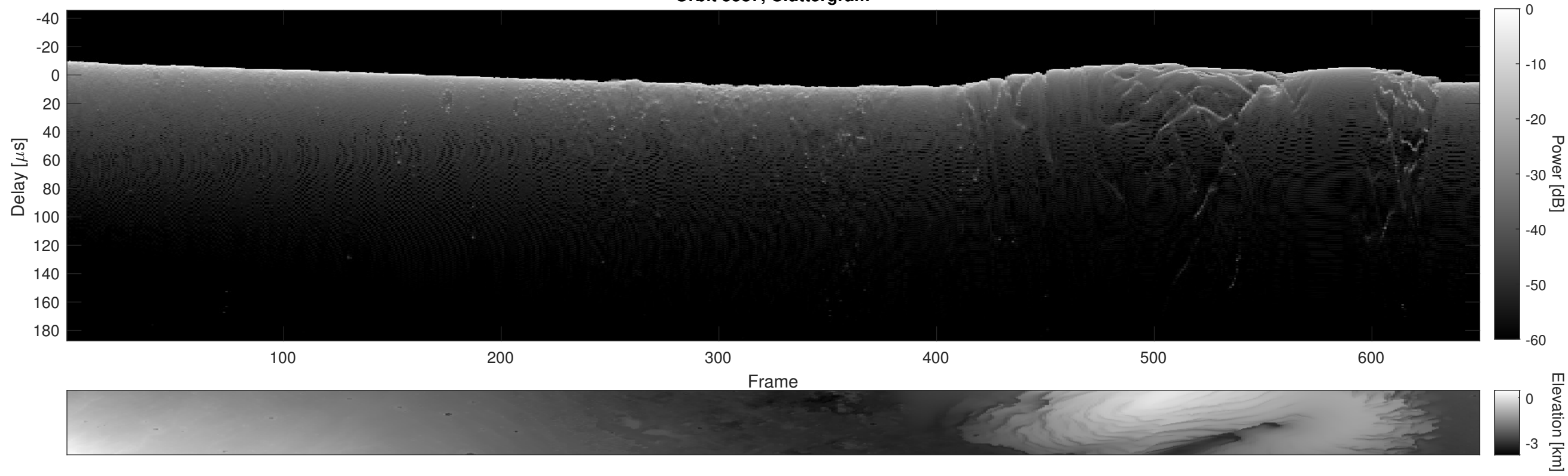
Orbit 5587, Cluttergram
