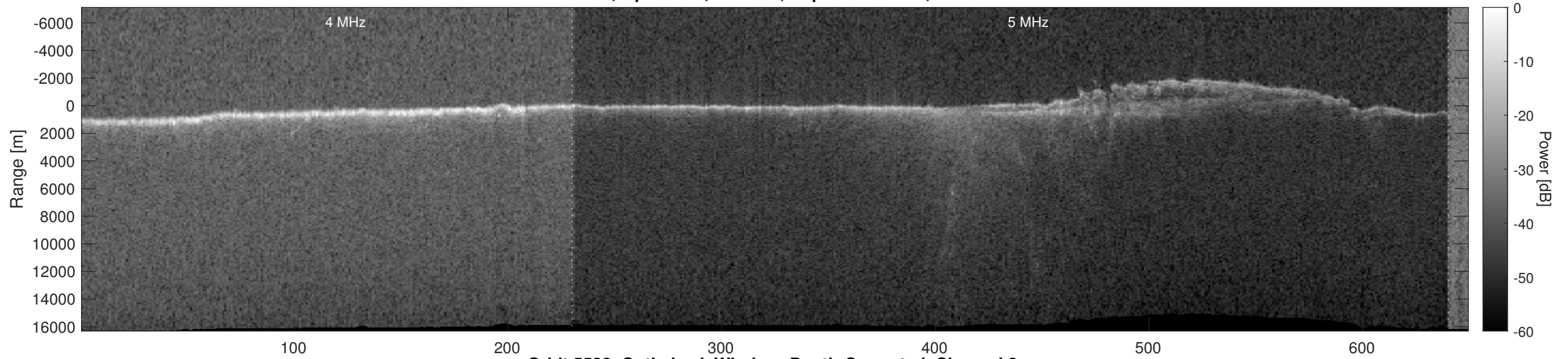
Orbit 5588, Optimized, Window, Depth-Corrected, Channel 2
