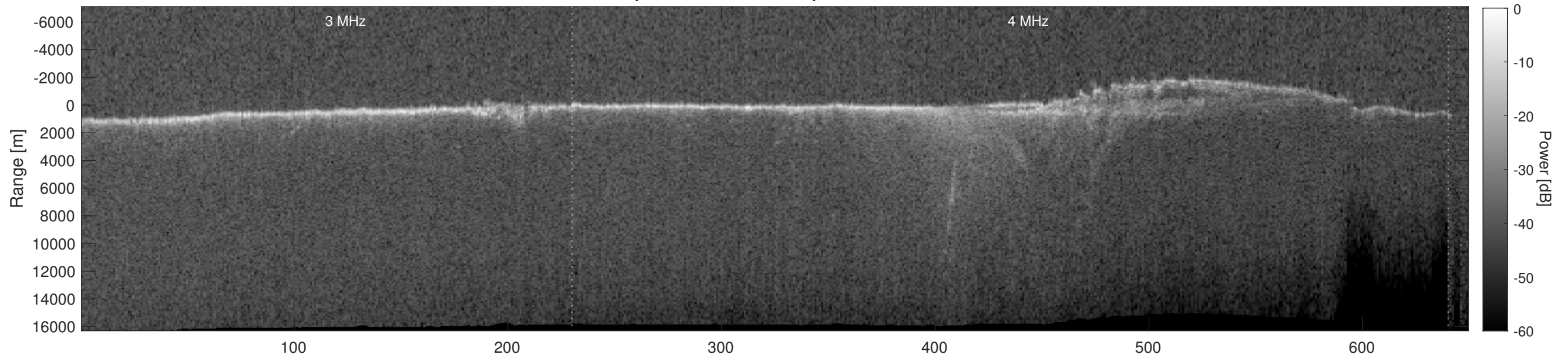
Orbit 5588, Depth-Corrected Cluttergram
