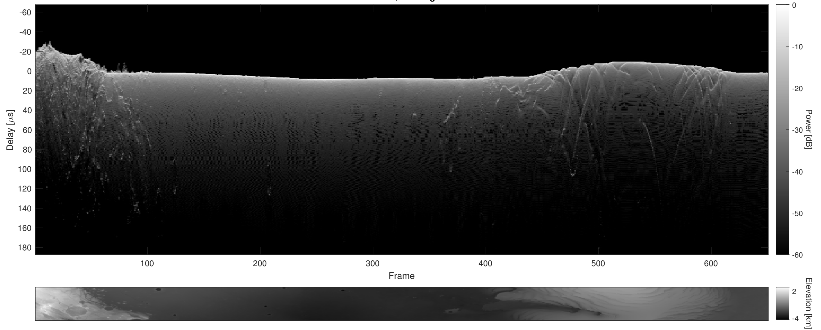
Orbit 5590, Cluttergram
