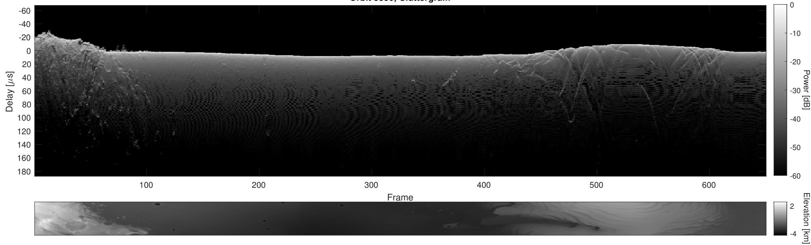
Orbit 5590, Cluttergram
