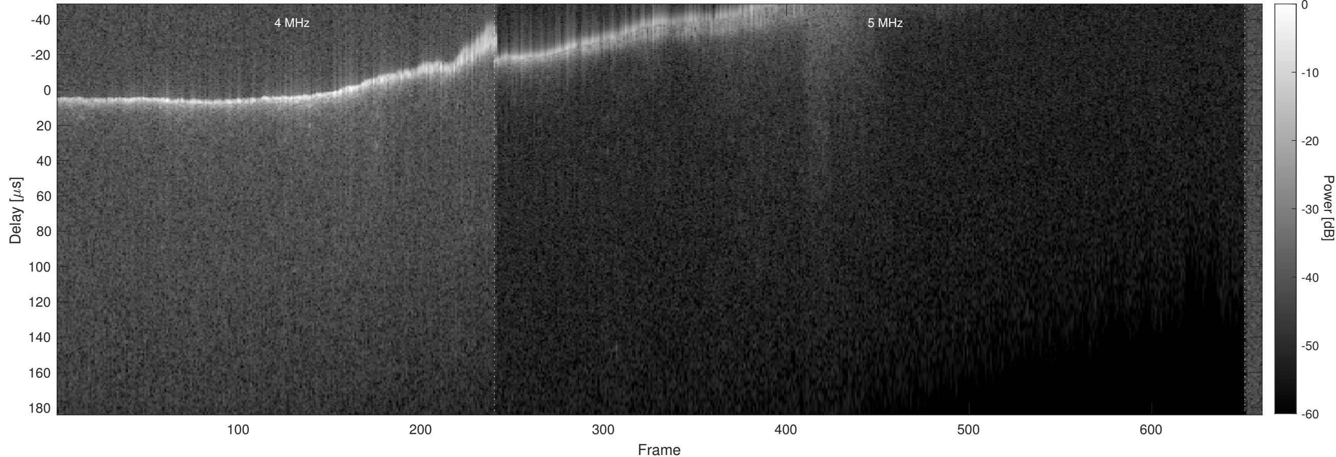
Orbit 5595, Chapman, No Window, Channel 2
