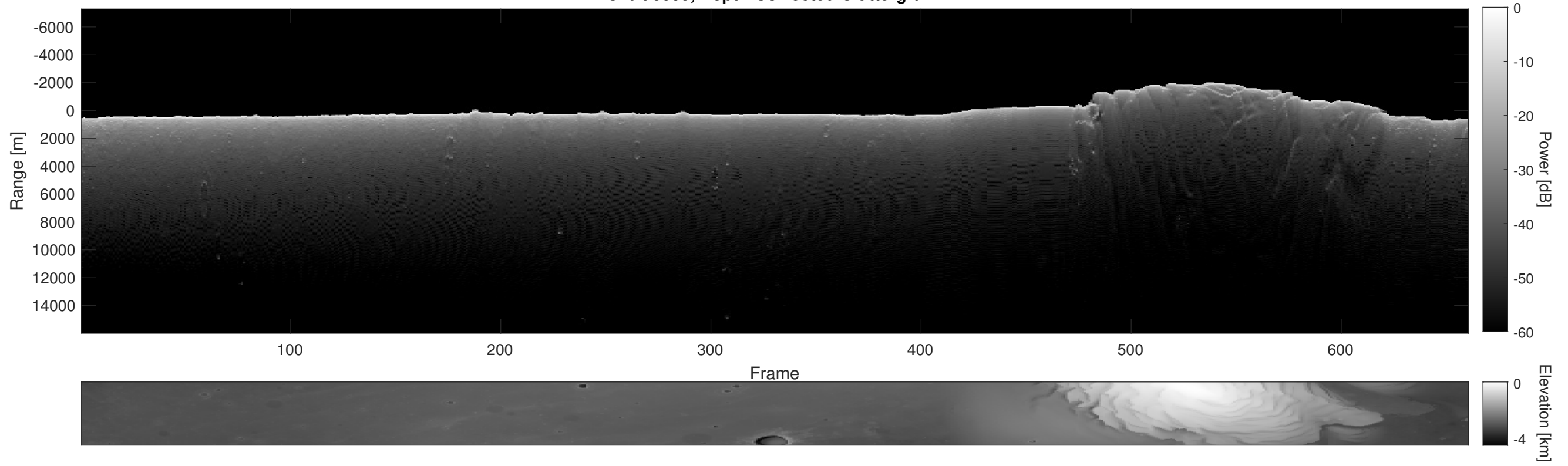
Orbit 5595, Depth-Corrected Cluttergram
