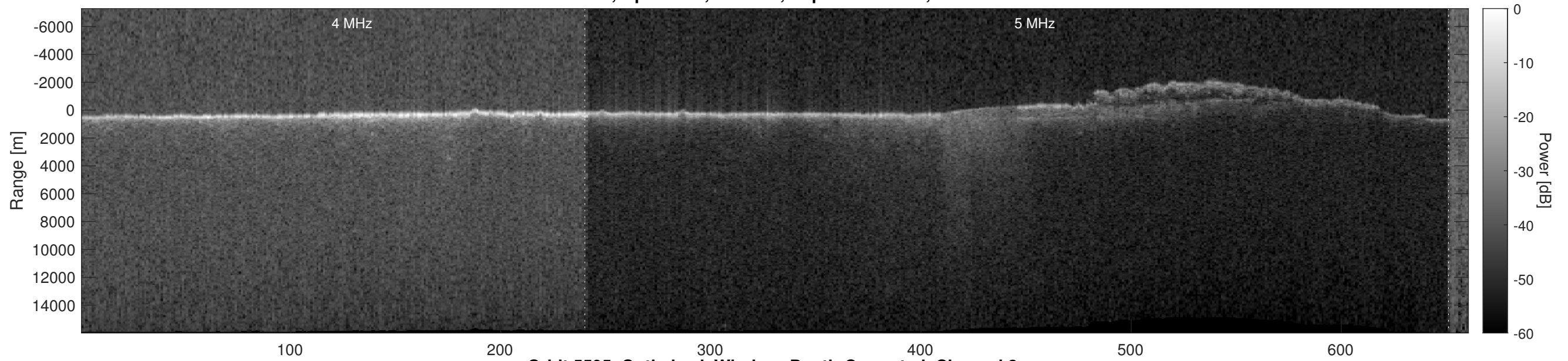
Orbit 5595, Optimized, Window, Depth-Corrected, Channel 2
