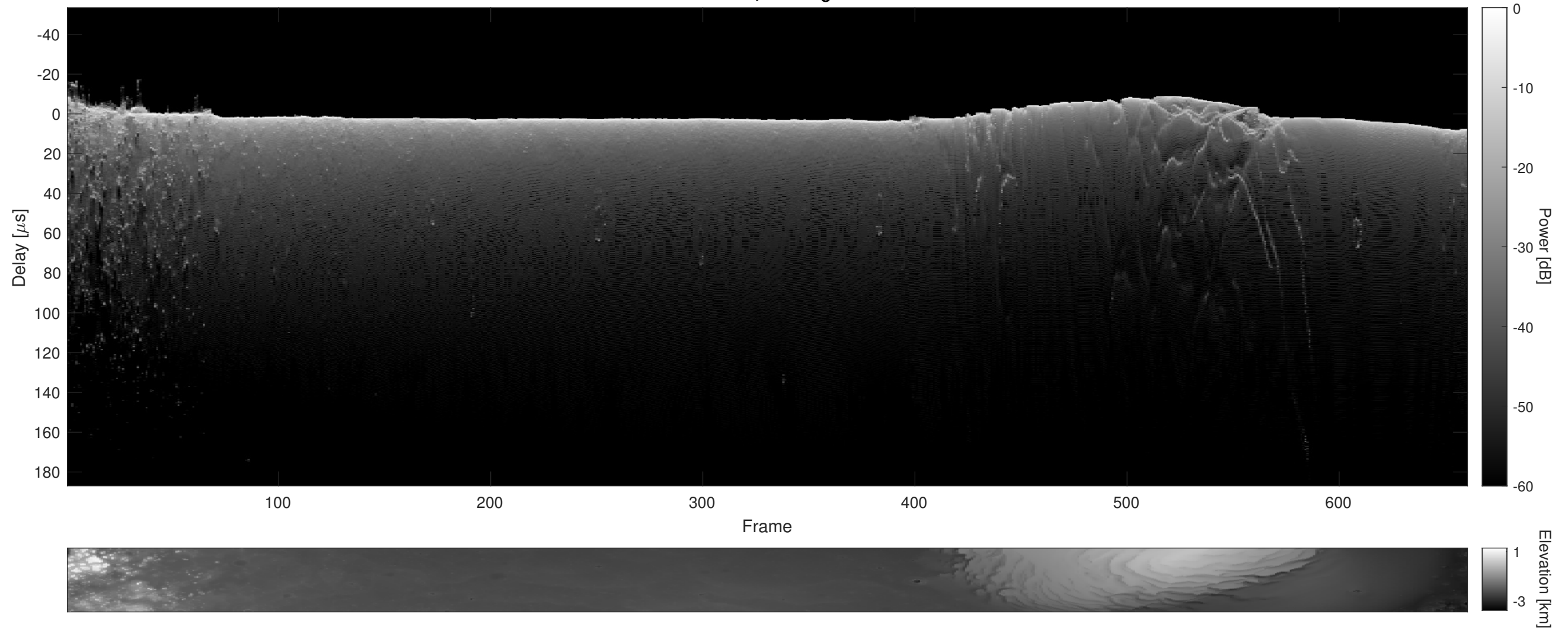
Orbit 5596, Cluttergram
