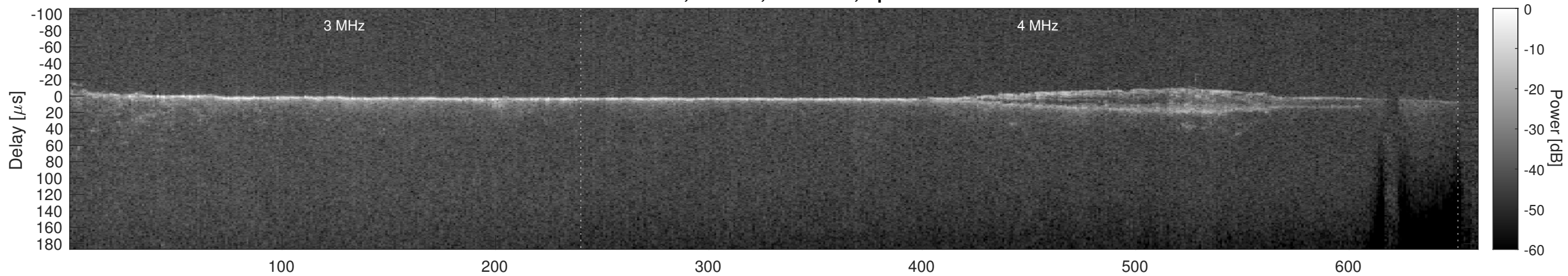
Orbit 5596, Cluttergram
