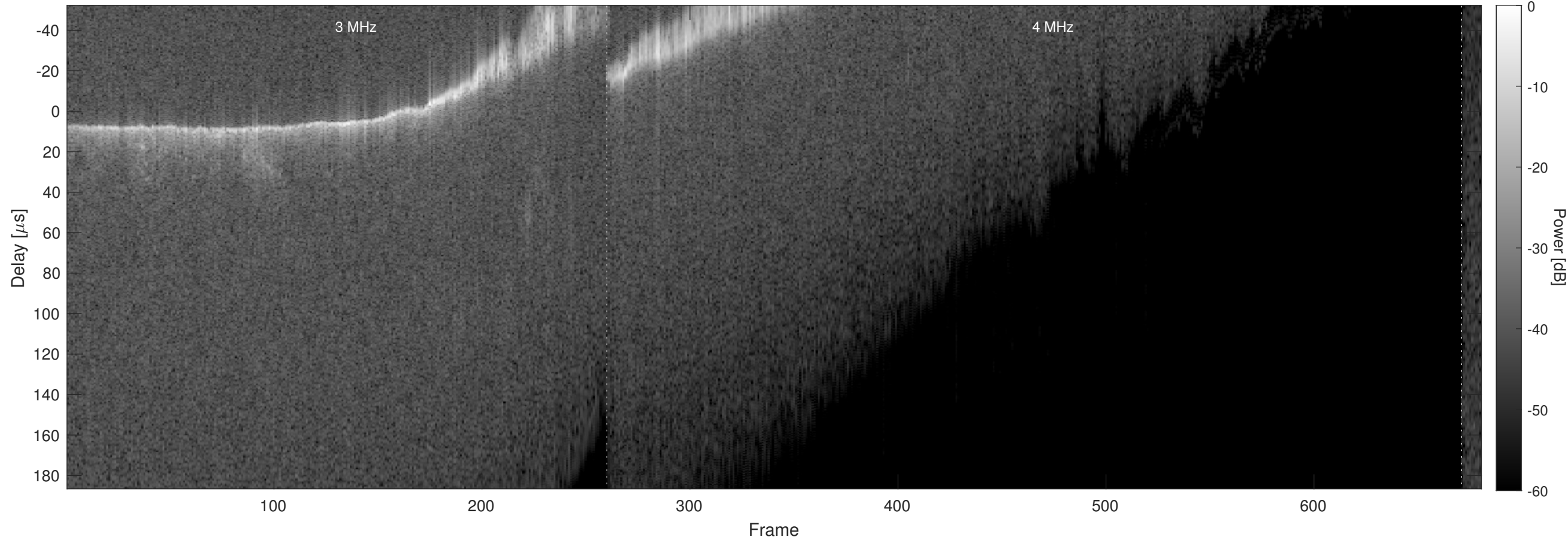
Orbit 5604, Chapman, No Window, Channel 2
