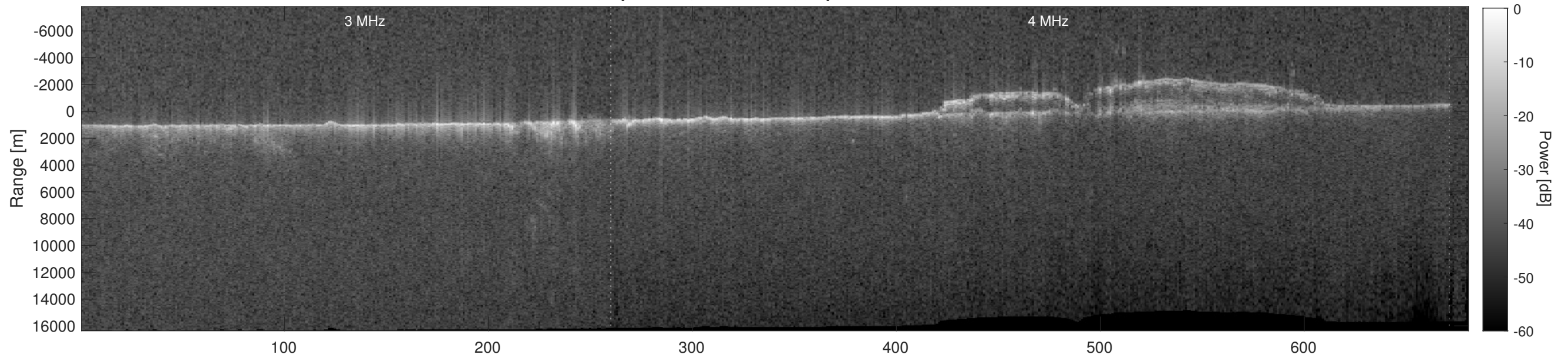
Orbit 5604, Depth-Corrected Cluttergram
