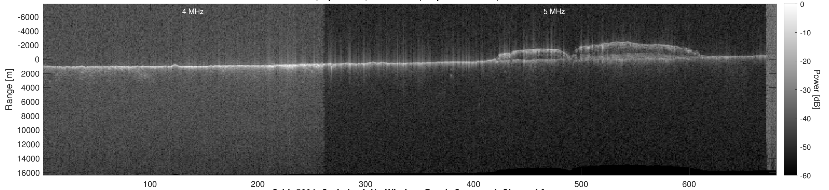
Orbit 5604, Optimized, No Window, Depth-Corrected, Channel 2
