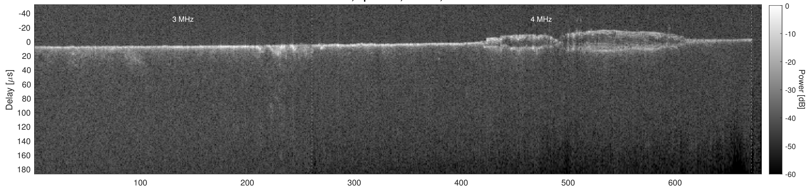
Orbit 5604, Cluttergram
