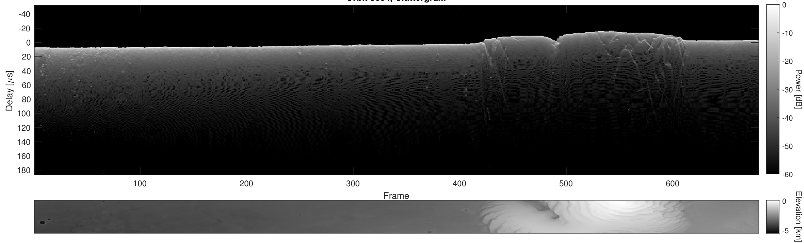
Orbit 5604, Cluttergram
