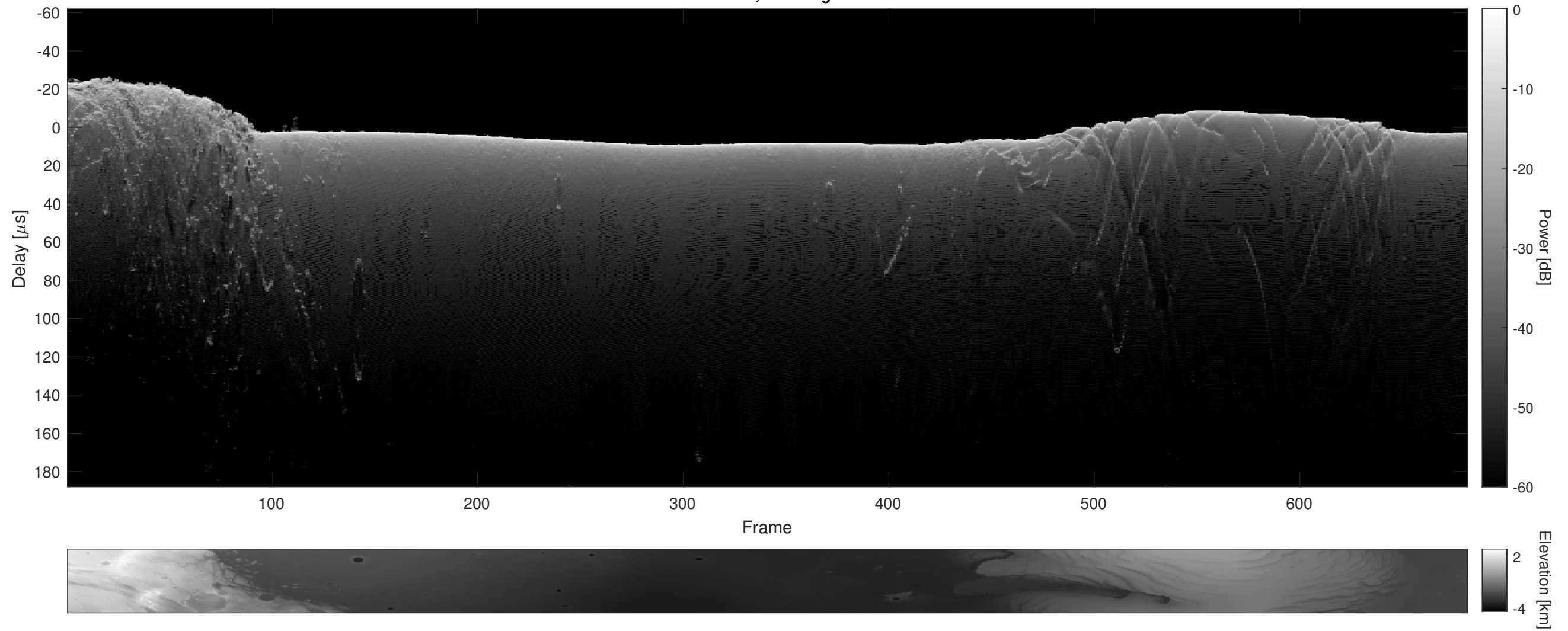
Orbit 5608, Cluttergram
