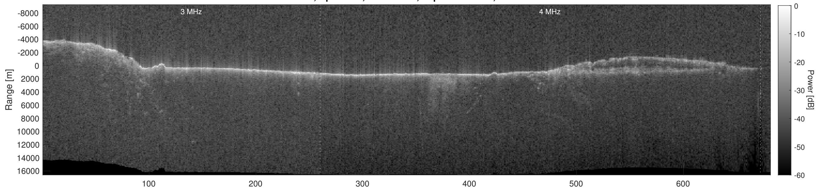
Orbit 5608, Depth-Corrected Cluttergram
