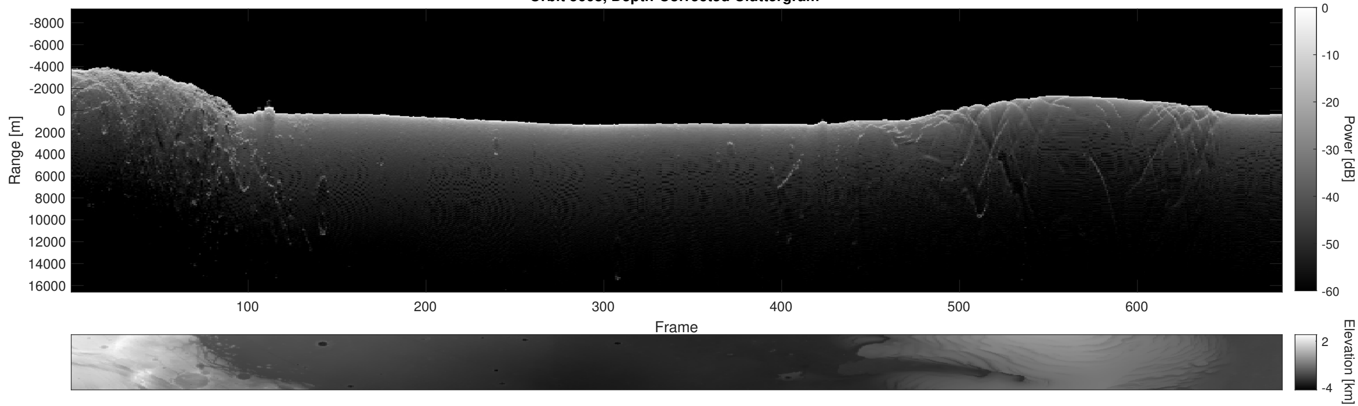
Orbit 5608, Depth-Corrected Cluttergram
