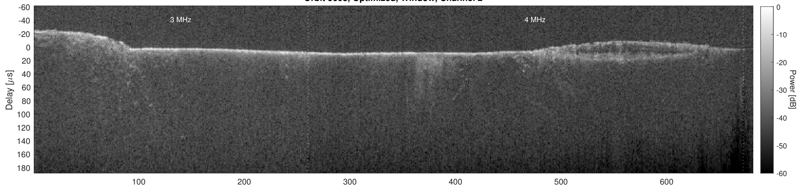
Orbit 5608, Cluttergram
