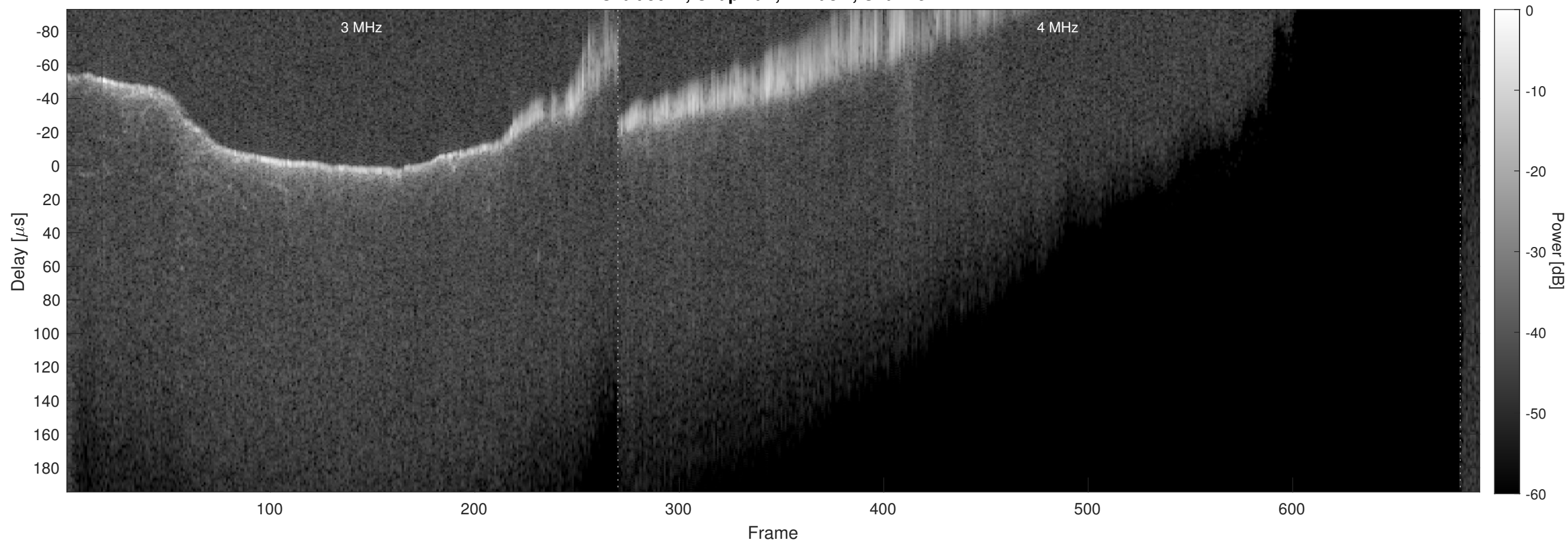
Orbit 5612, Chapman, Window, Channel 2
