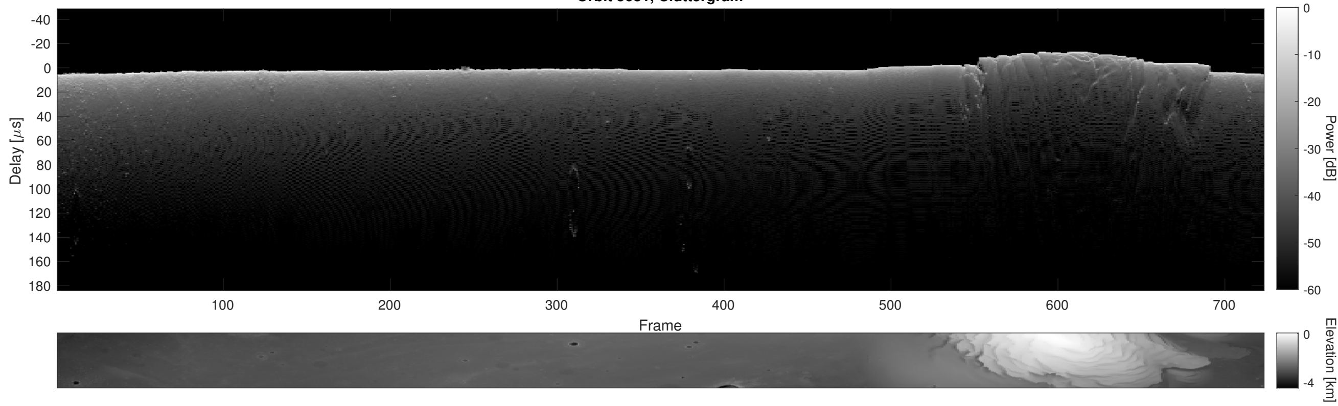
Orbit 5631, Cluttergram
