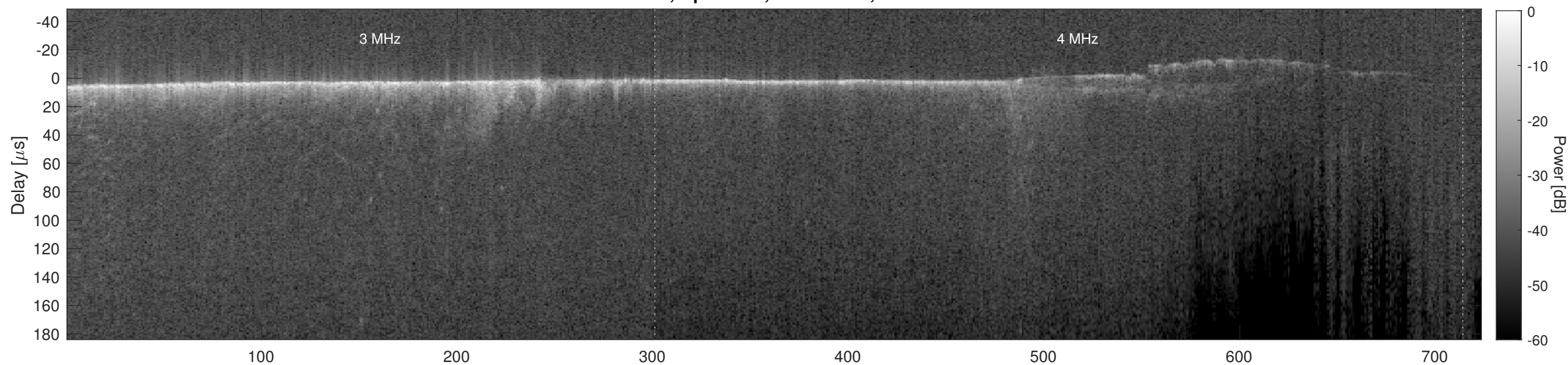
Orbit 5631, Cluttergram
