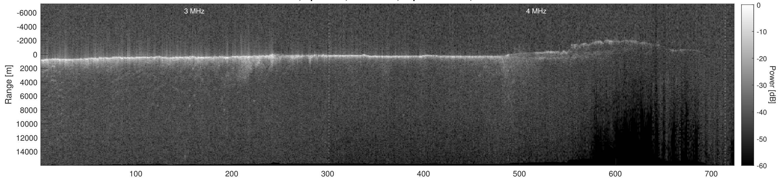
Orbit 5631, Depth-Corrected Cluttergram
