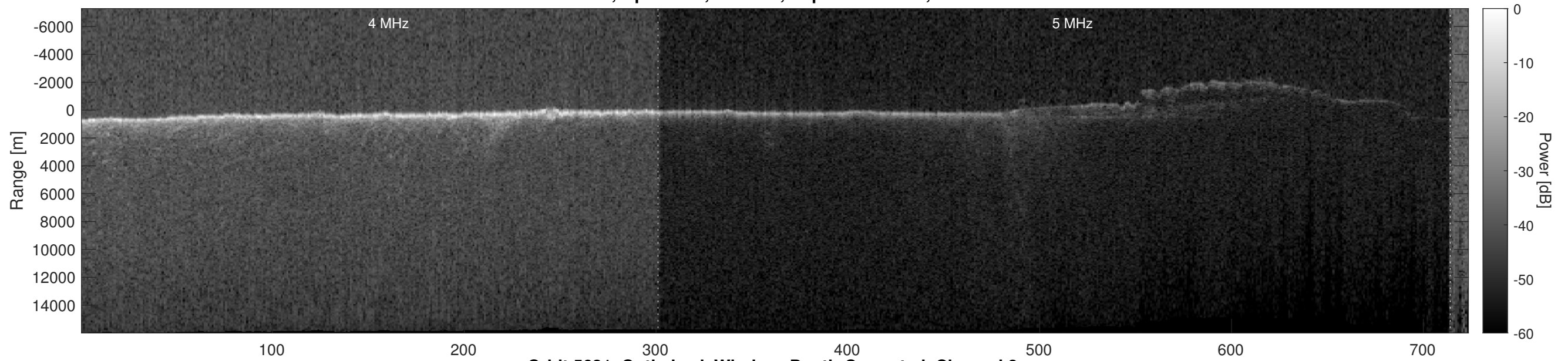
Orbit 5631, Optimized, Window, Depth-Corrected, Channel 2
