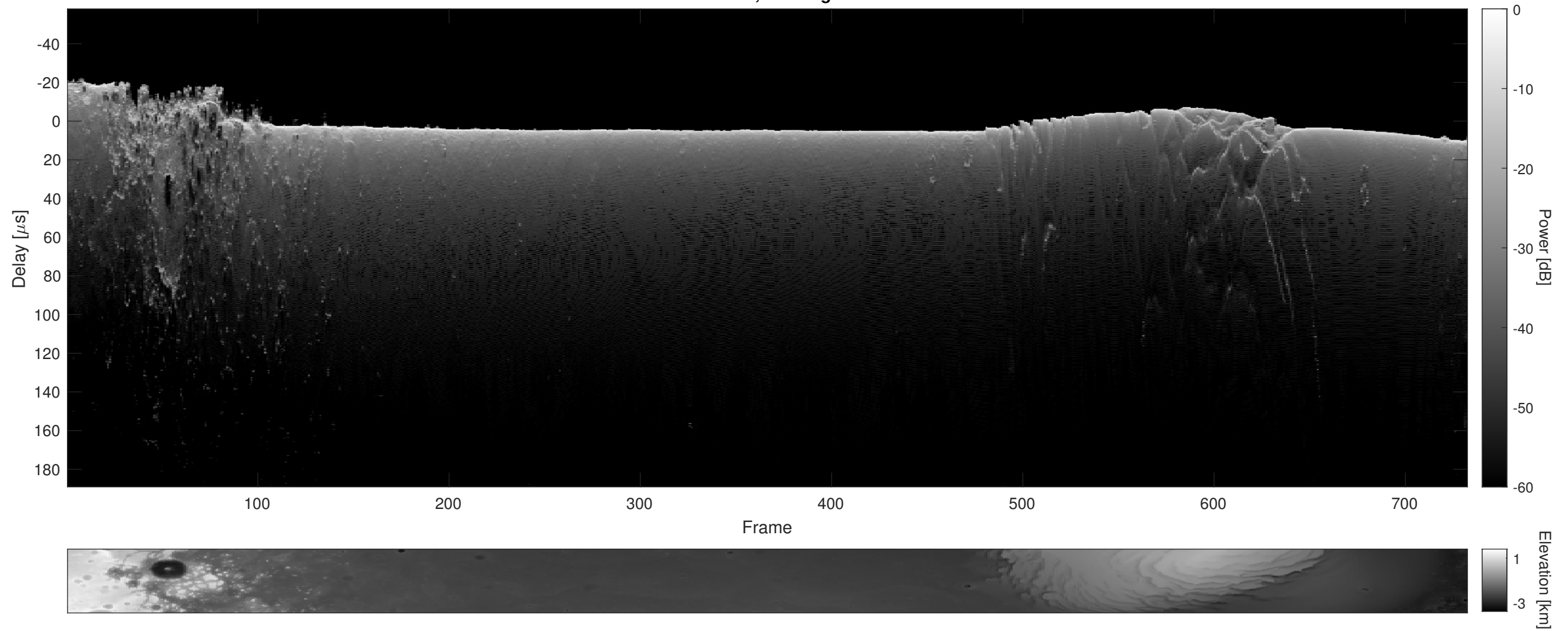
Orbit 5632, Cluttergram
