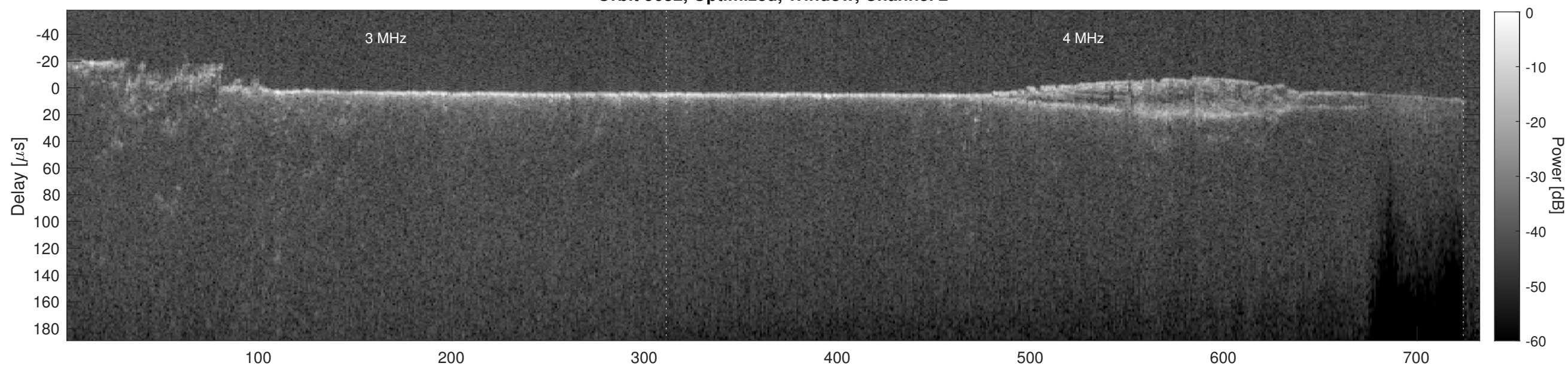
Orbit 5632, Cluttergram
