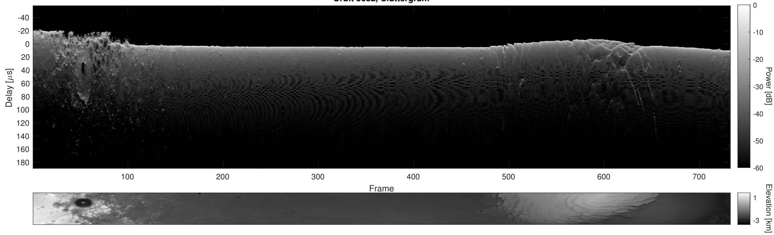
Orbit 5632, Cluttergram
