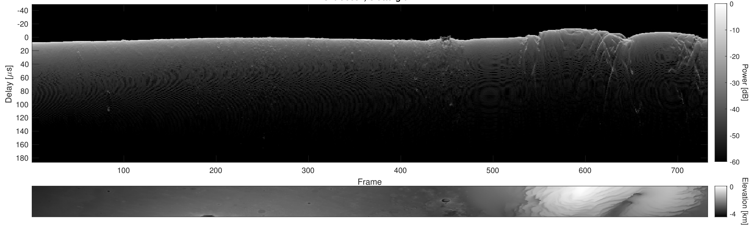
Orbit 5634, Cluttergram
