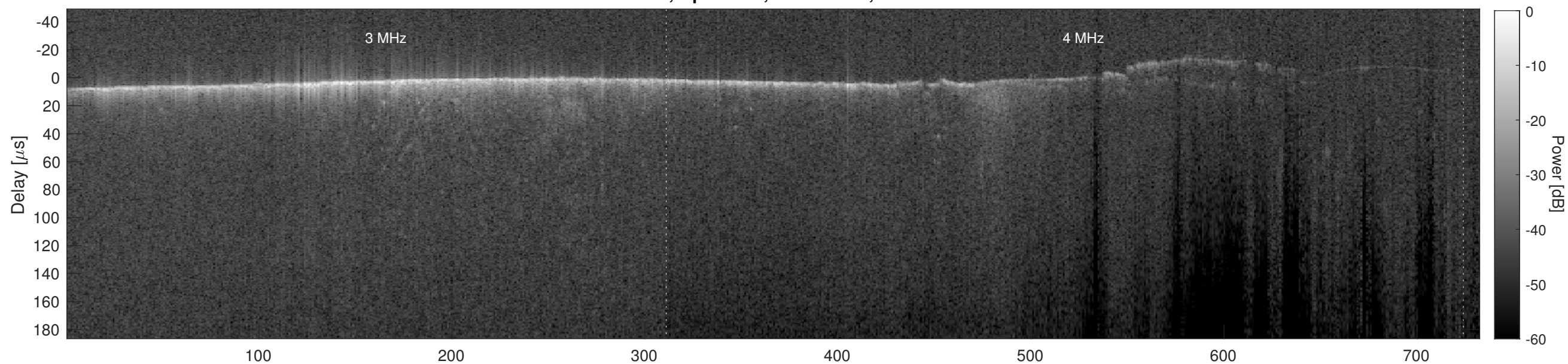
Orbit 5634, Cluttergram
