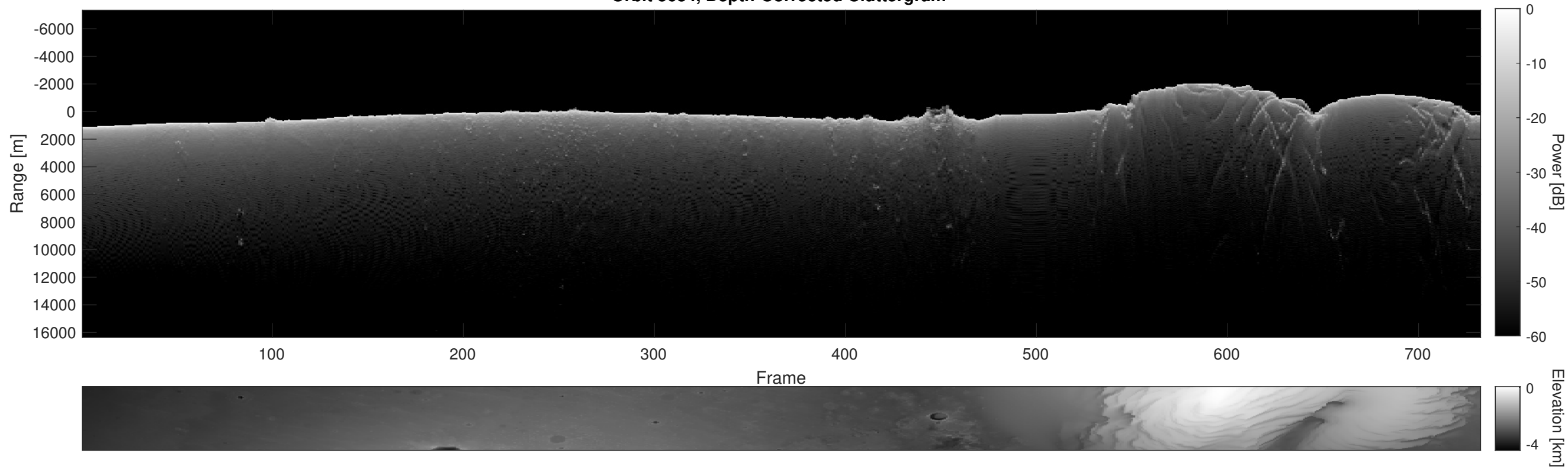
Orbit 5634, Depth-Corrected Cluttergram
