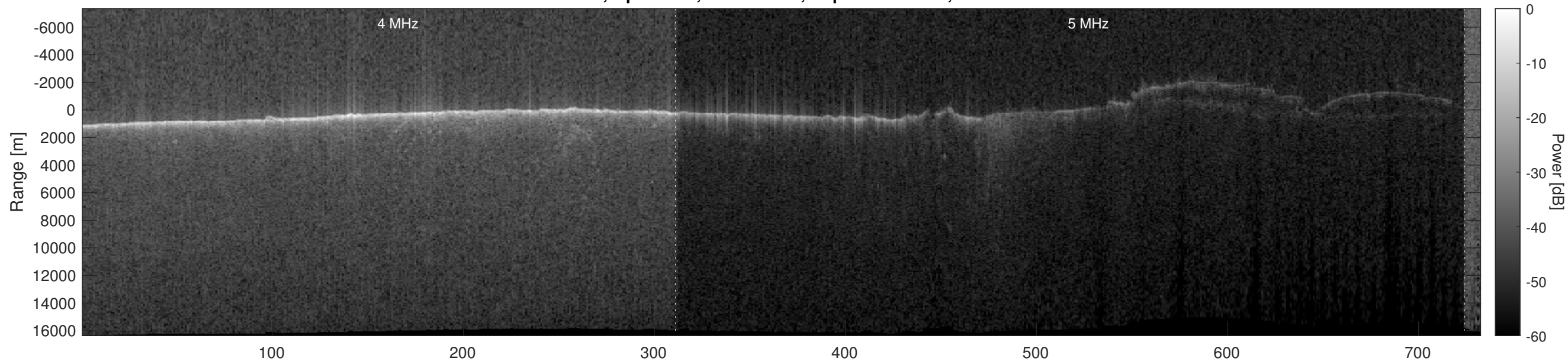
Orbit 5634, Optimized, No Window, Depth-Corrected, Channel 2
