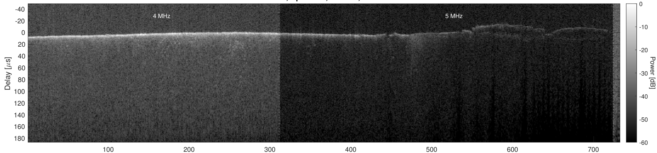
Orbit 5634, Optimized, Window, Channel 2
