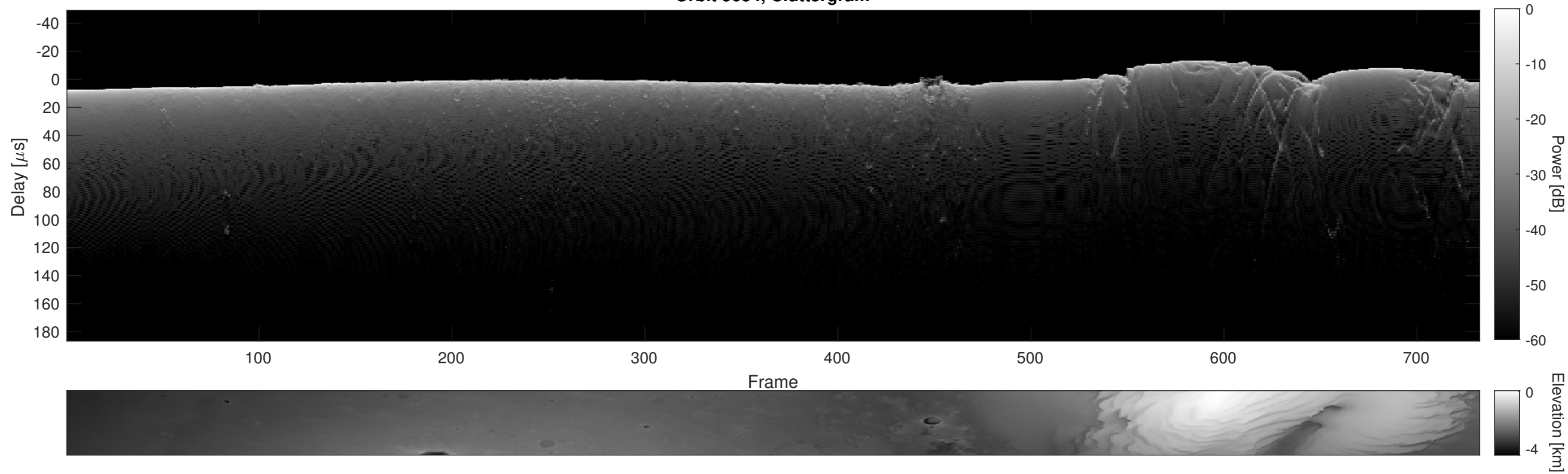
Orbit 5634, Cluttergram
