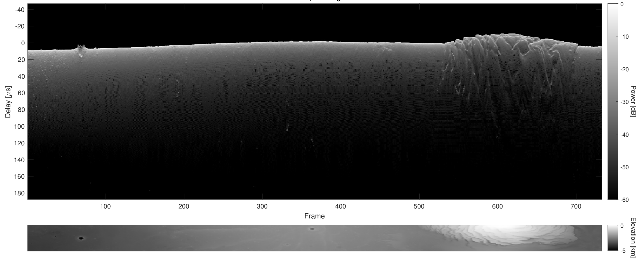
Orbit 5635, Cluttergram
