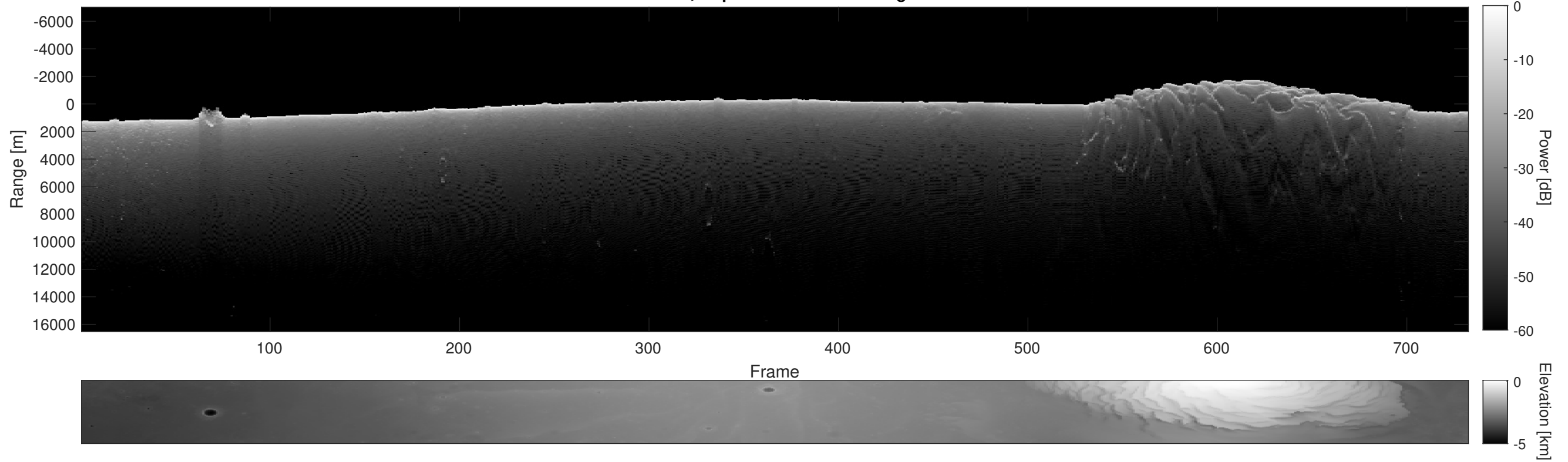
Orbit 5635, Depth-Corrected Cluttergram
