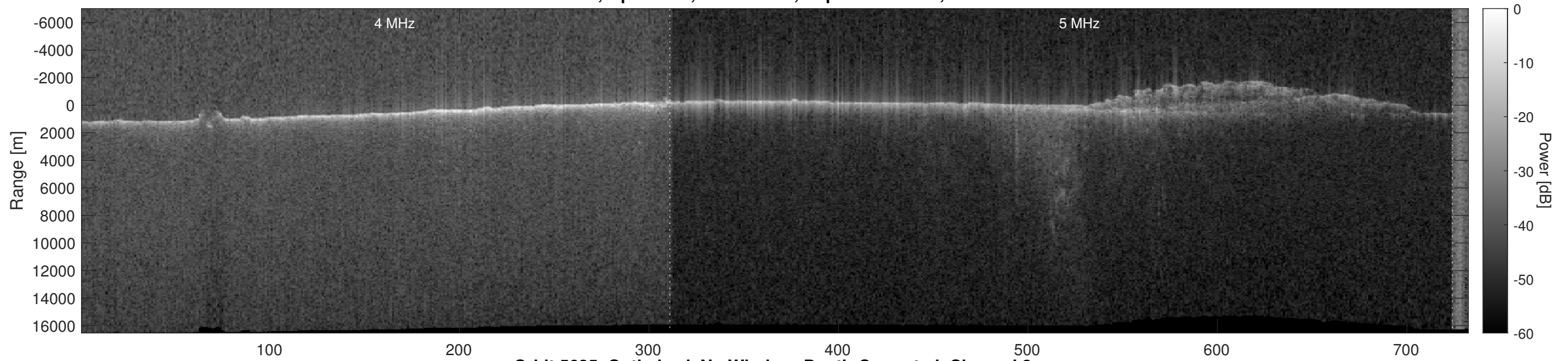
Orbit 5635, Optimized, No Window, Depth-Corrected, Channel 2
