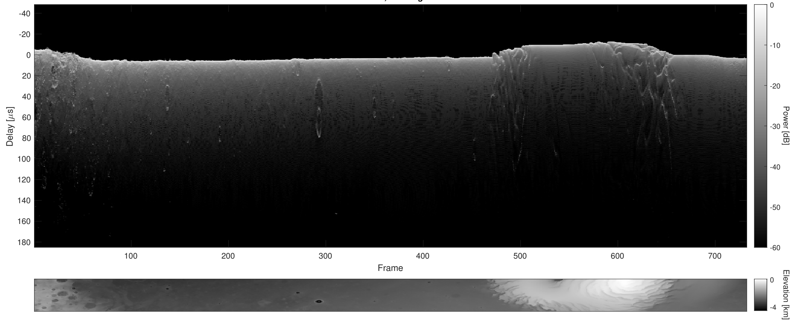
Orbit 5636, Cluttergram
