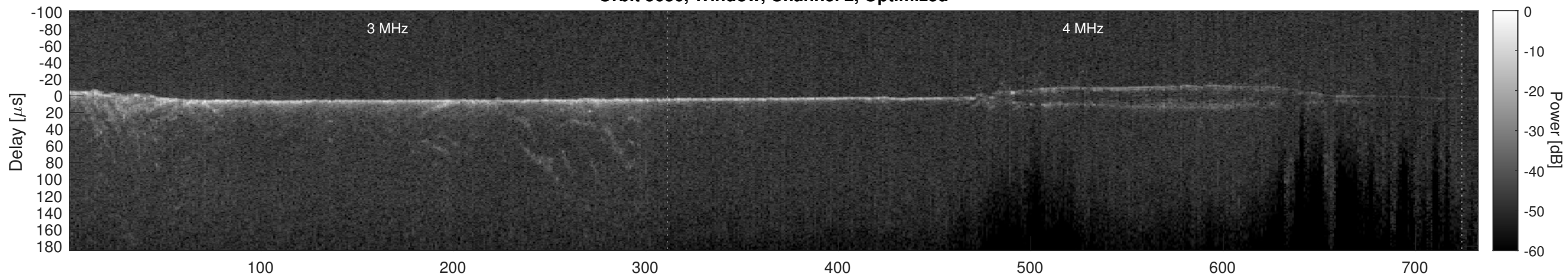
Orbit 5636, Cluttergram
