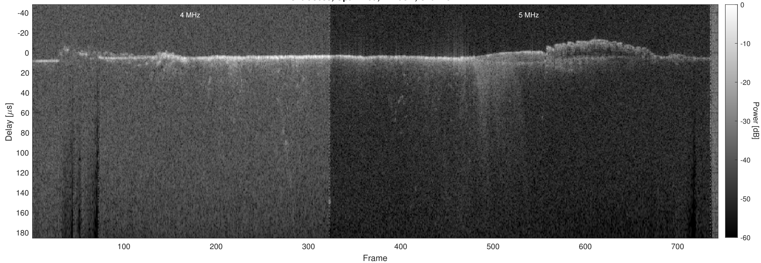
Orbit 5638, Optimized, Window, Channel 2
