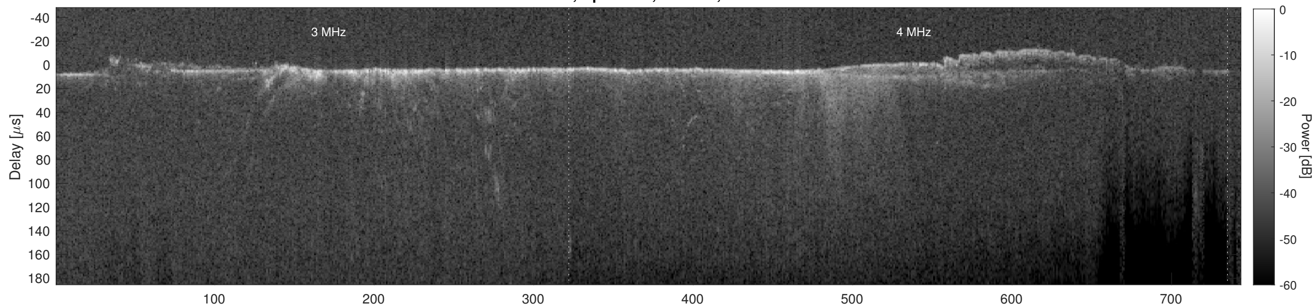
Orbit 5638, Cluttergram
