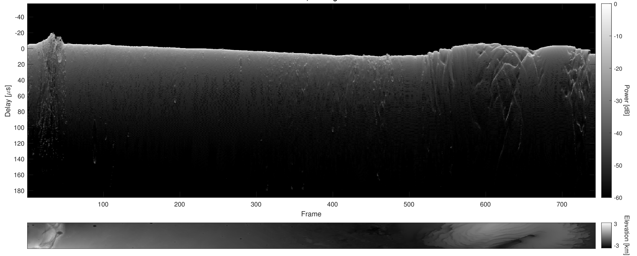
Orbit 5641, Cluttergram
