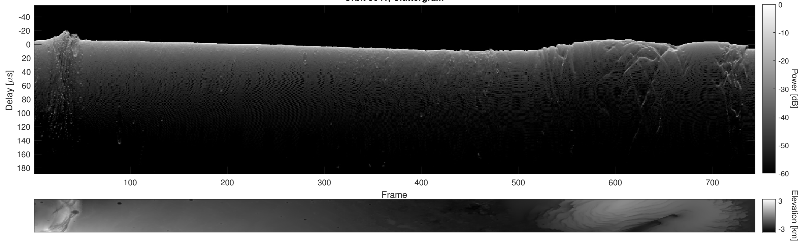
Orbit 5641, Cluttergram
