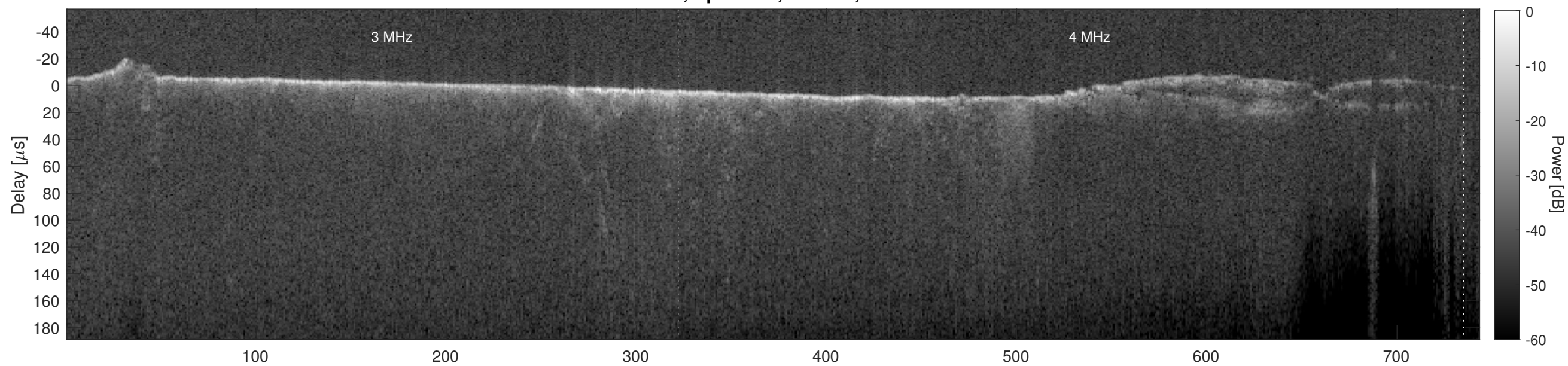
Orbit 5641, Cluttergram
