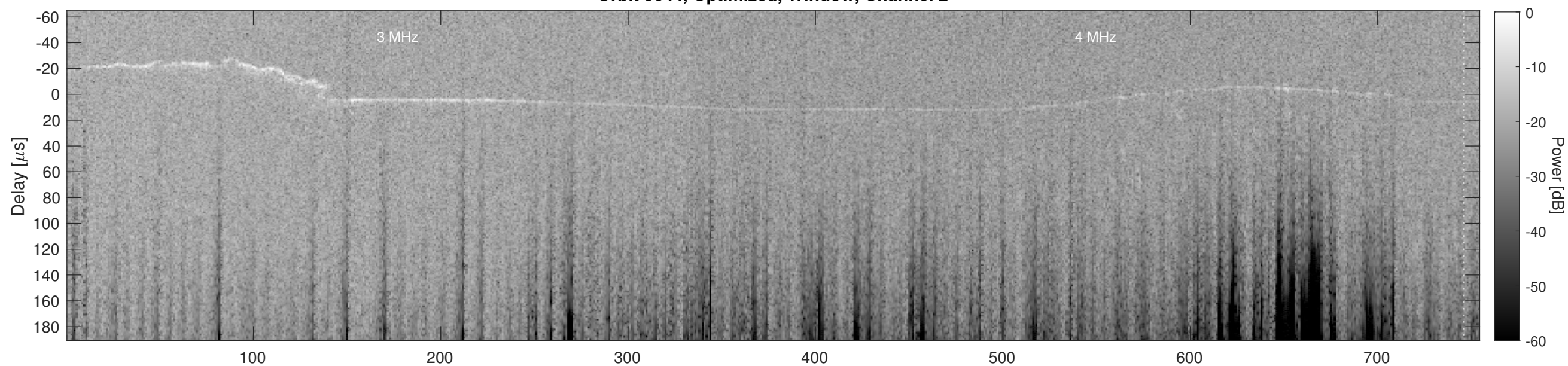
Orbit 5644, Cluttergram
