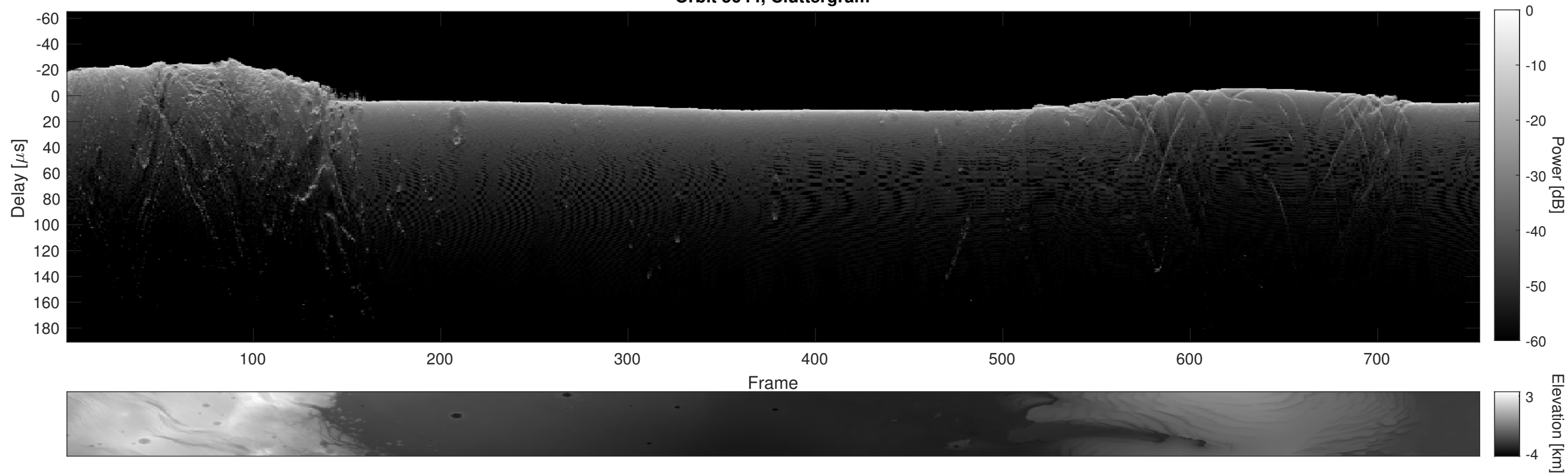
Orbit 5644, Cluttergram
