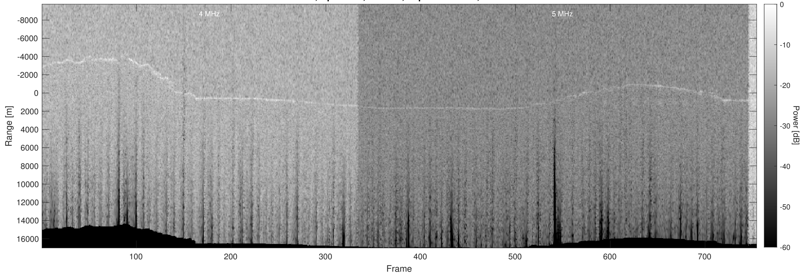
Orbit 5644, Optimized, Window, Depth-Corrected, Channel 2
