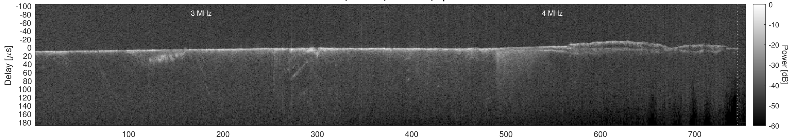
Orbit 5645, Cluttergram
