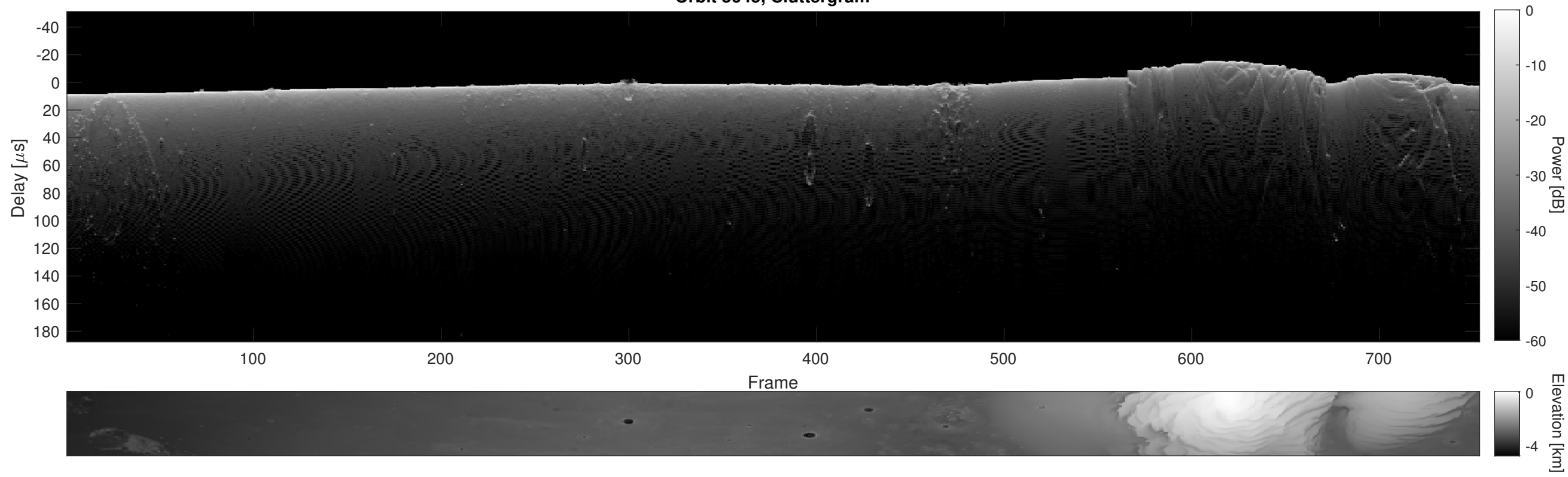
Orbit 5645, Cluttergram
