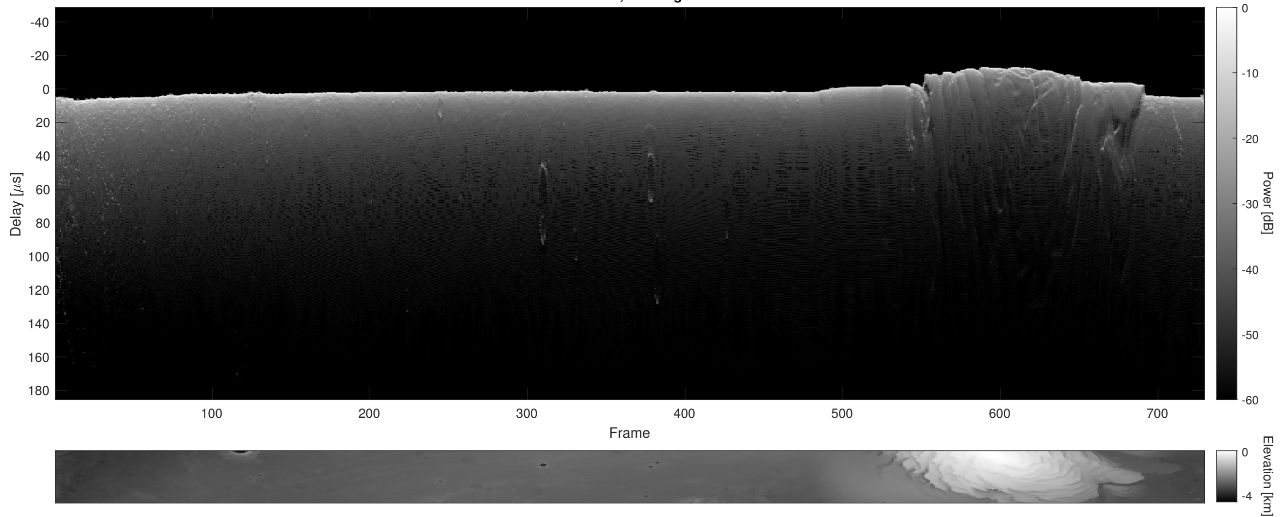
Orbit 5649, Cluttergram
