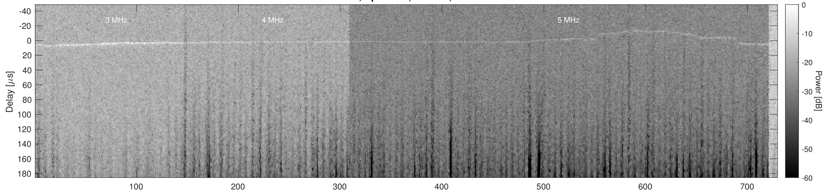
Orbit 5649, Optimized, Window, Channel 2
