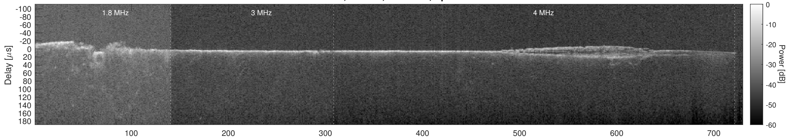
Orbit 5650, Cluttergram
