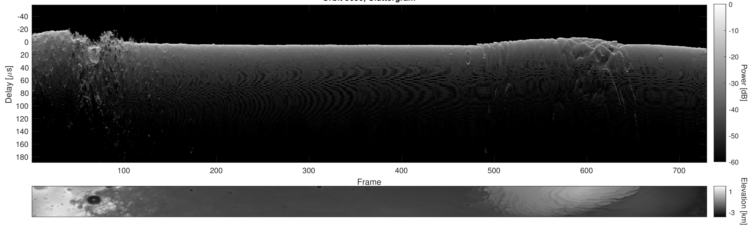
Orbit 5650, Cluttergram
