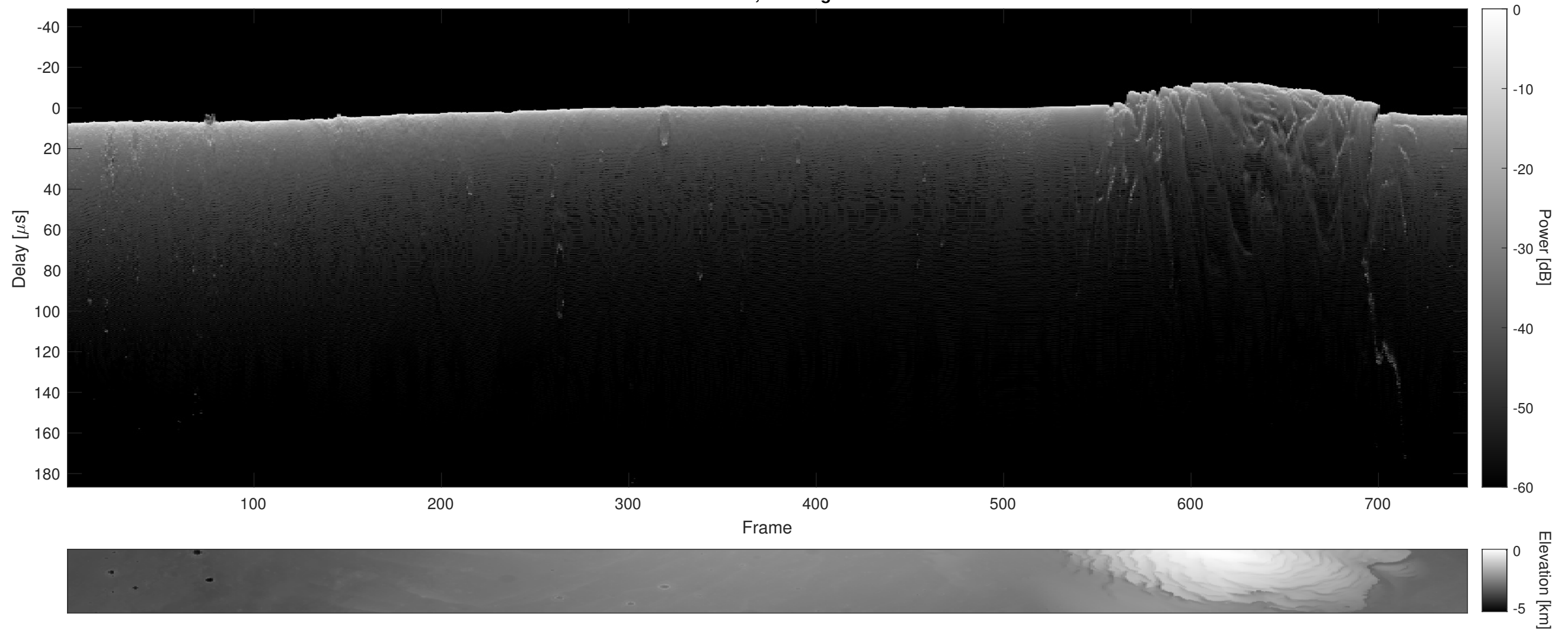
Orbit 5660, Cluttergram
