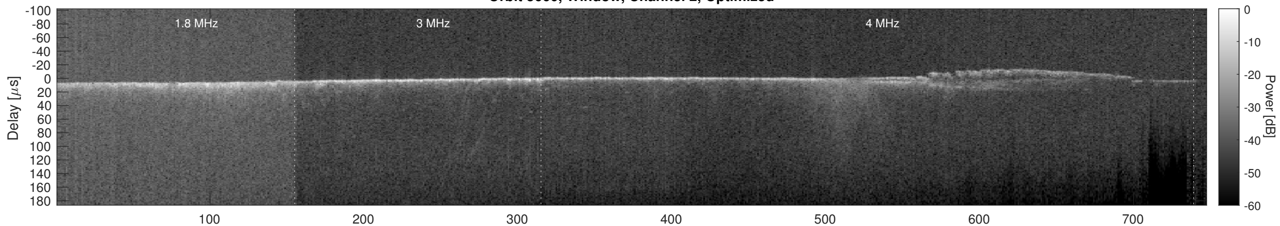
Orbit 5660, Cluttergram
