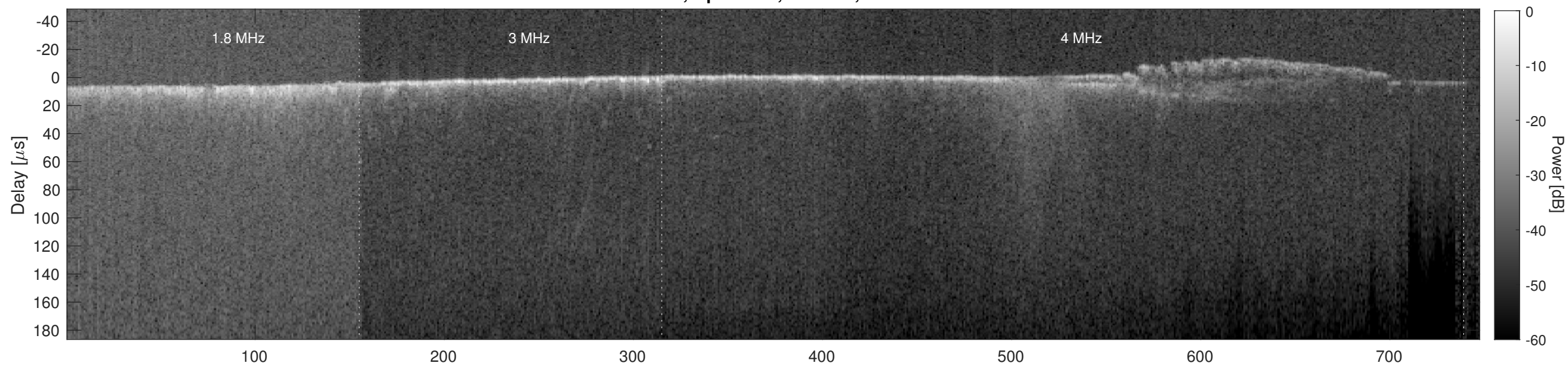
Orbit 5660, Cluttergram
