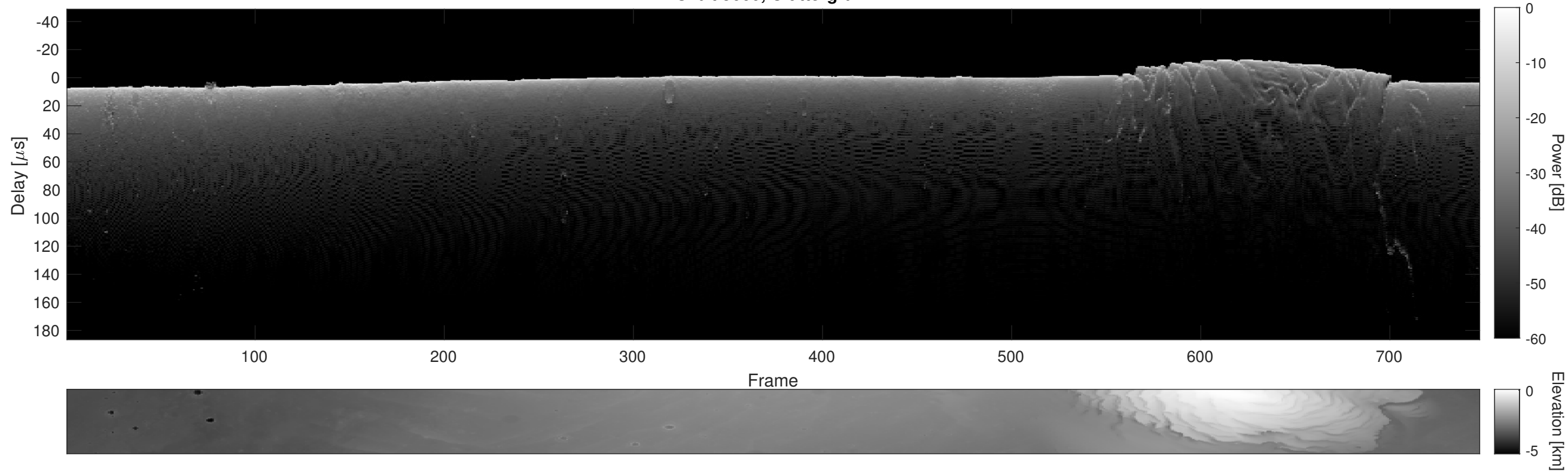
Orbit 5660, Cluttergram
