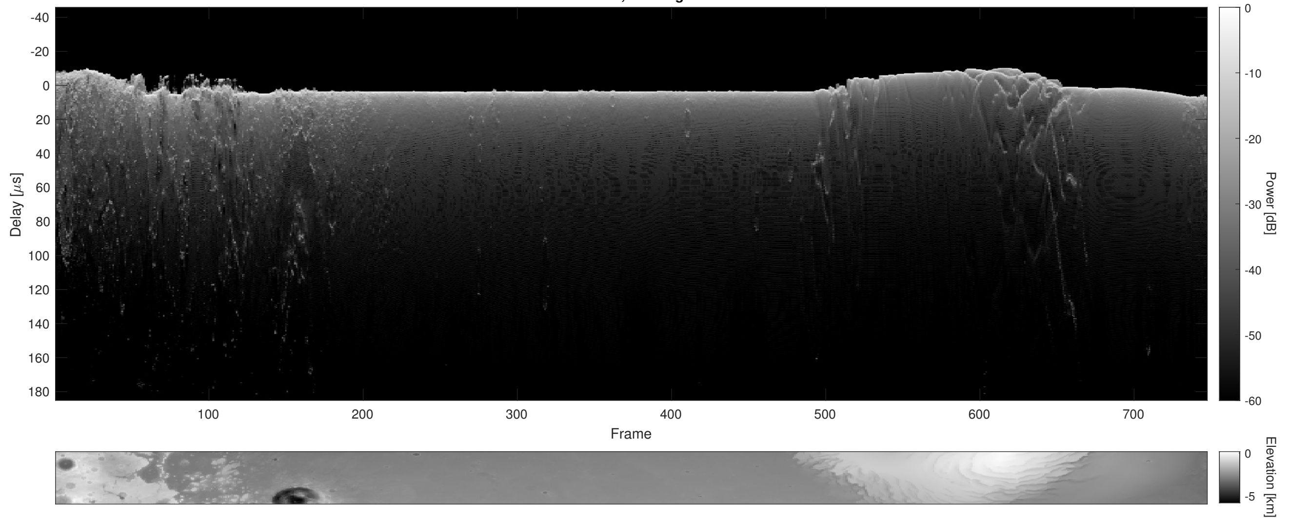
Orbit 5661, Cluttergram
