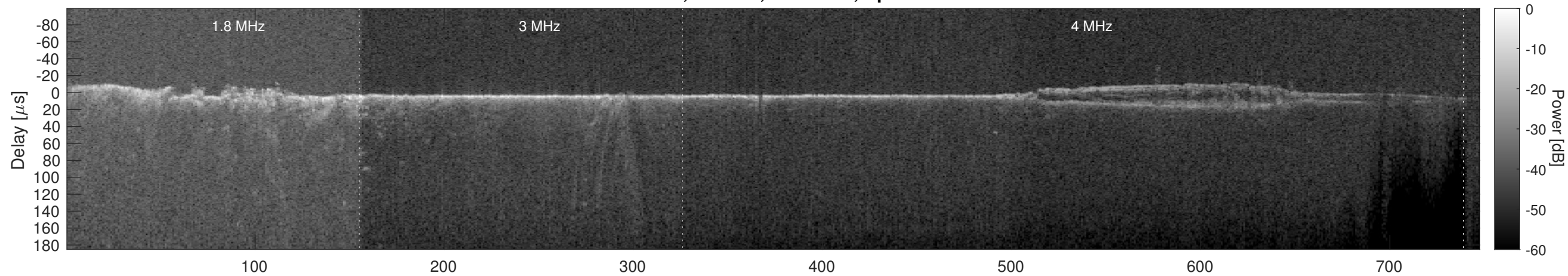
Orbit 5661, Cluttergram
