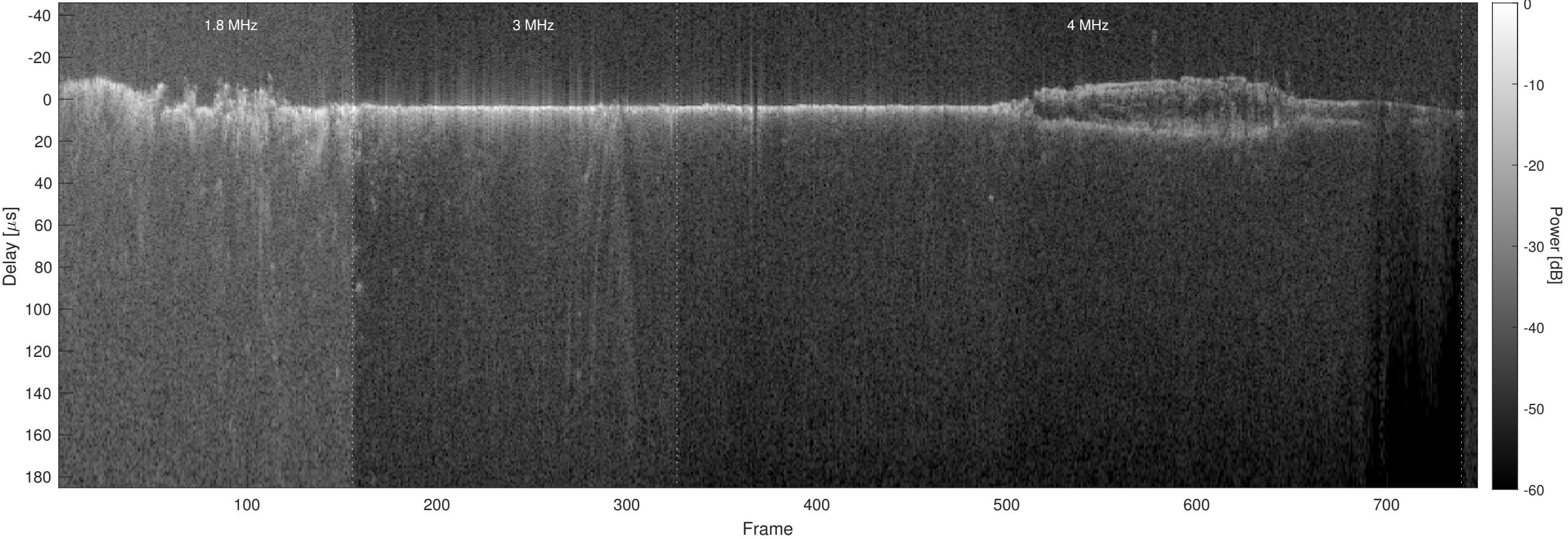
Orbit 5661, Optimized, No Window, Channel 2
