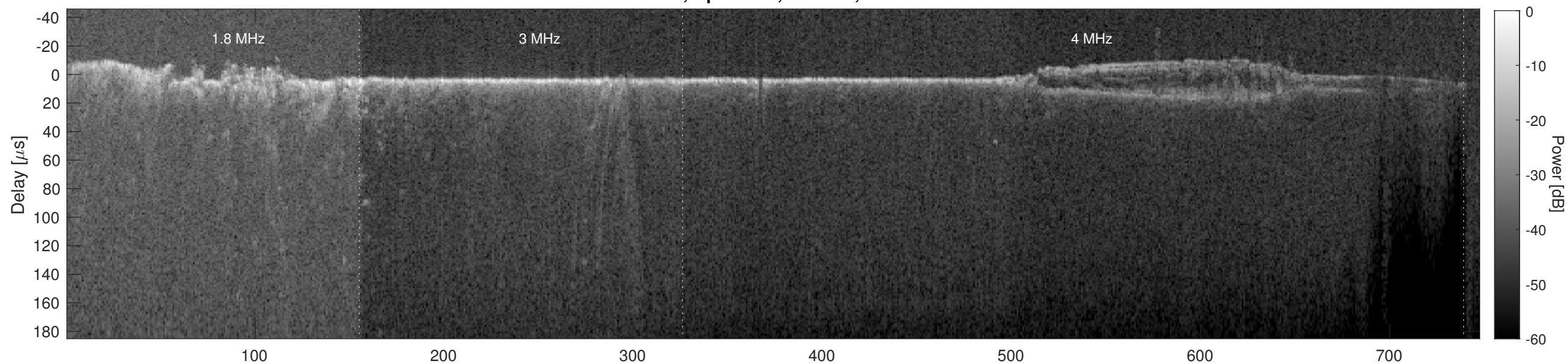
Orbit 5661, Cluttergram
