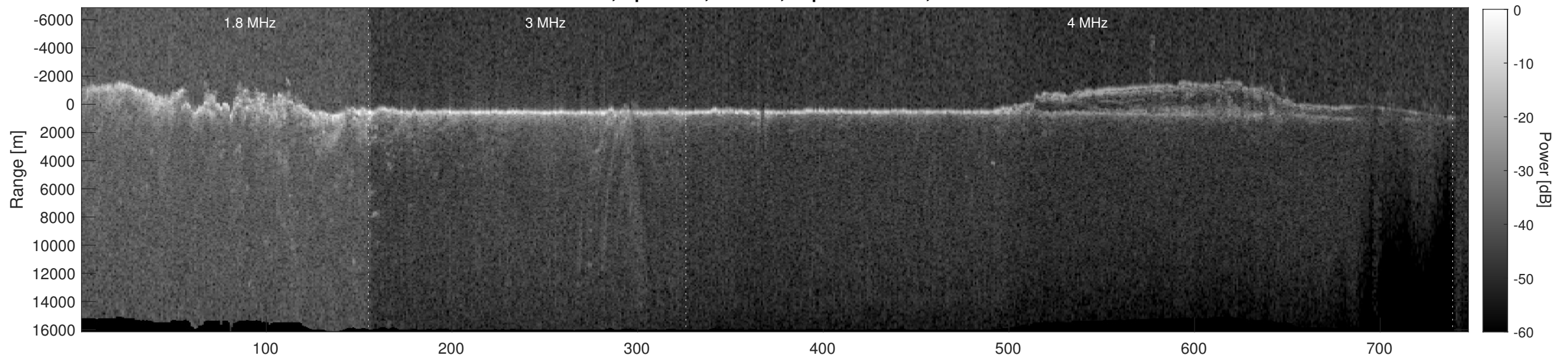
Orbit 5661, Depth-Corrected Cluttergram
