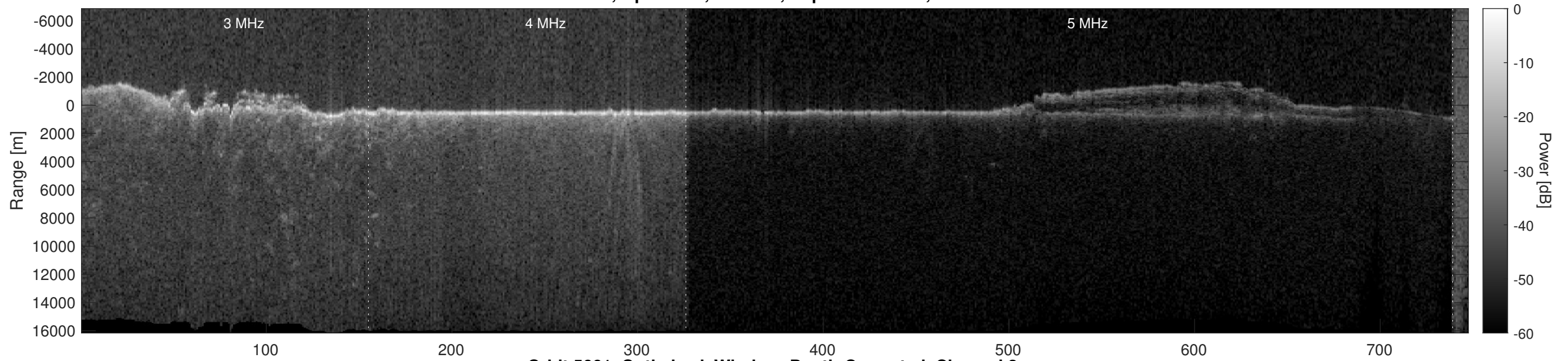
Orbit 5661, Optimized, Window, Depth-Corrected, Channel 2
